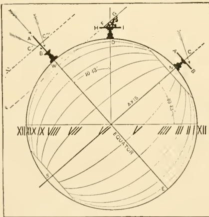
Fig. 5—The Earth, Showing Relation of Dial Styles to Axis
